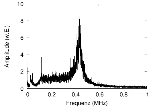
Abb. 3.16: LVF3c: Fourier-Spektrum.
