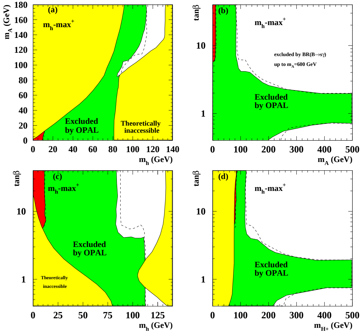
Figure 6.11: Results for the “ m_h -max ^+ ” benchmark scenario described in the text of Section 6.4.1. See Fig. 6.8 for the notation.
