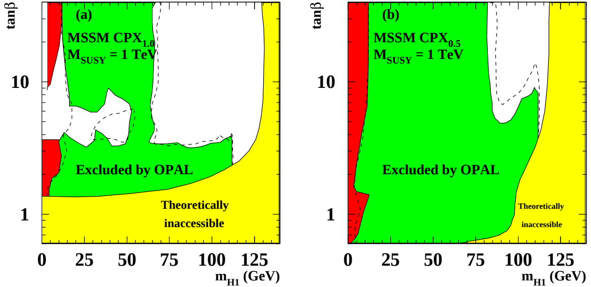
Figure 6.22: The “CPX” MSSM 95 % CL exclusion areas in the (m_{H_1}, \tan\beta) plane, using scans (a) preserving the “CPX” ratios of \mu , A_{b,t} and m_{\text{SUSY}} , using m_{\text{SUSY}} = 1 TeV, and (b) m_{\text{SUSY}} = 1 TeV keeping \mu and A_{b,t} at their “CPX” values. See Fig. 6.8 for the notation.
