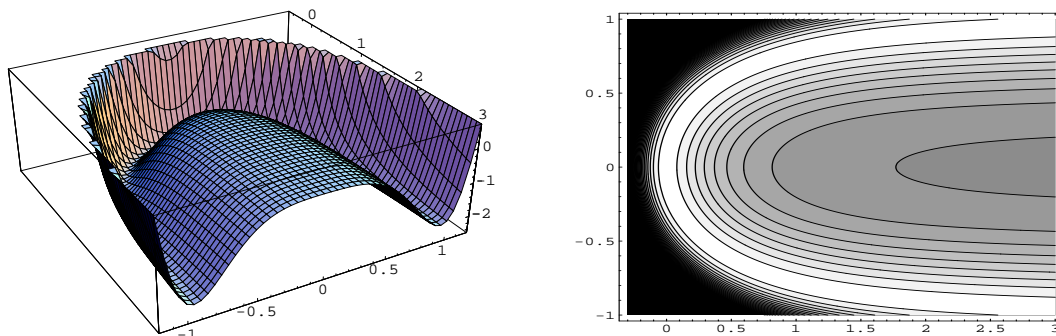
Figure 5.1: Flat valley in the potential, the \mathcal{N} = (4, 4) origin is located at (0, 0) . Coordinates here are x = \sin \phi \sinh z , y = \cos \phi \sinh z .
