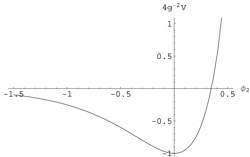
Figure 3.1: The scalar potential for the gauge group singlets
