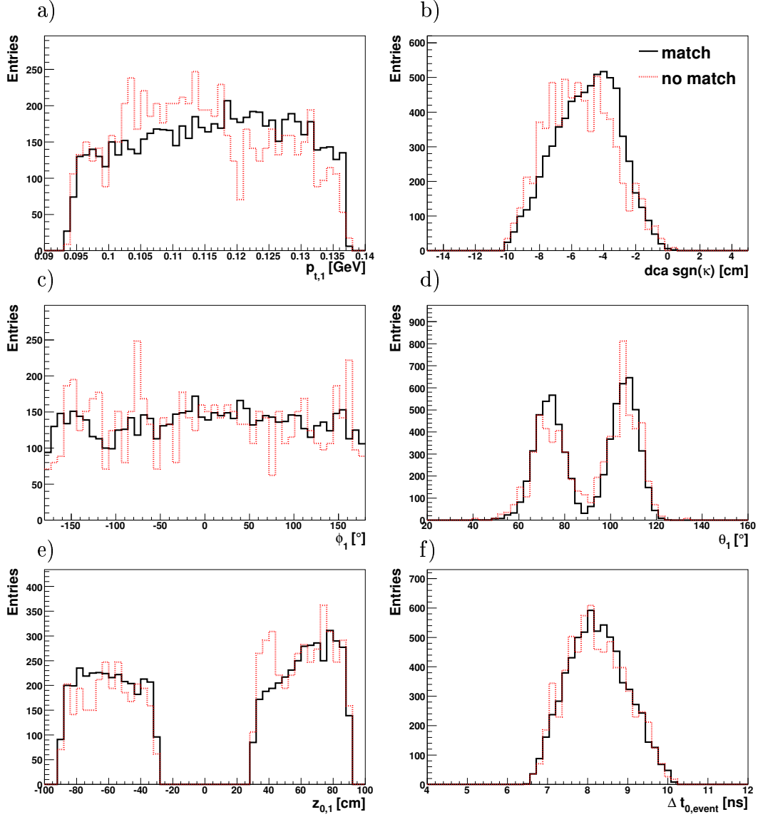
Figure B.5: Distributions in the track parameters p_{t1} , dca , \phi_1 , \theta_1 , z_{01} and \Delta t_{0,event} for the CJC2 curlers in comparison with and without matched second track. The distributions are area normalized.
