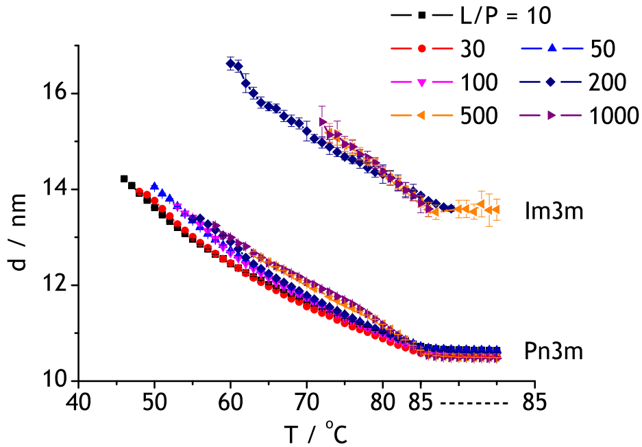
Figure 3.45: Lattice parameters of cubic phases in POPE-alamethicin mixtures during heating. The POPE to alamethicin ratios L/P are indicated.
