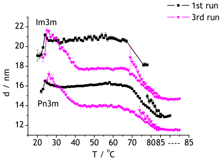
Figure 3.27: Lattice parameters of the cubic phases in the sample mm during the first and the third measurement.
