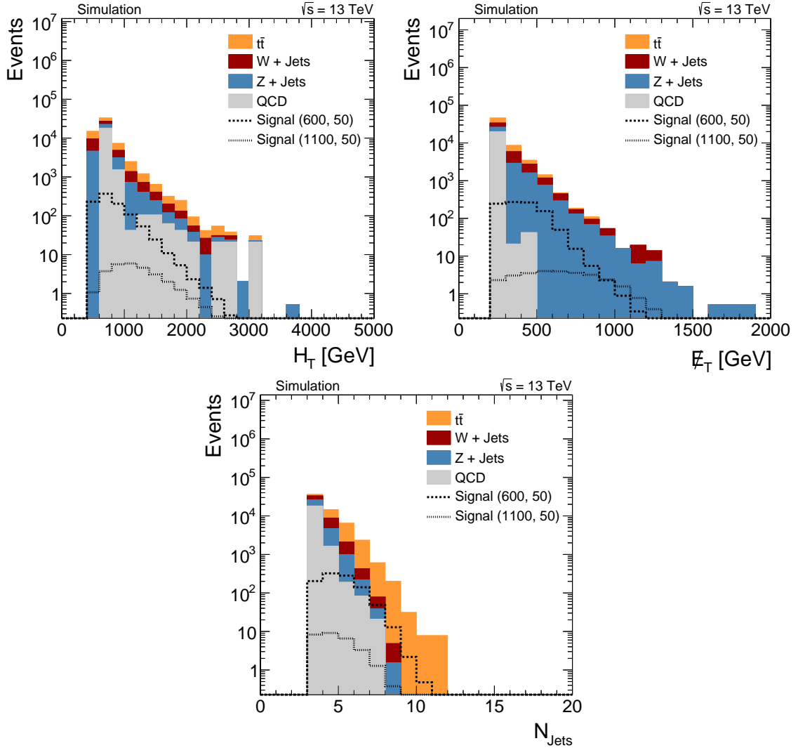
Figure 8.1: Comparison of selected H_T ( top left ), \cancel{E}_T ( top right ) and N_{\text{Jets}} ( bottom ) distributions in simulated events found from applying the baseline selection criteria. The signal points are labelled as (X, Y) where X is the top squark mass and Y is the LSP mass in GeV.
