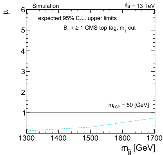
Figure 8.19: Expected 95% C.L. upper limit for signal strength versus m_{\tilde{g}} . The LSP mass is chosen to be 50 GeV. The label B. denotes the baseline selection.
