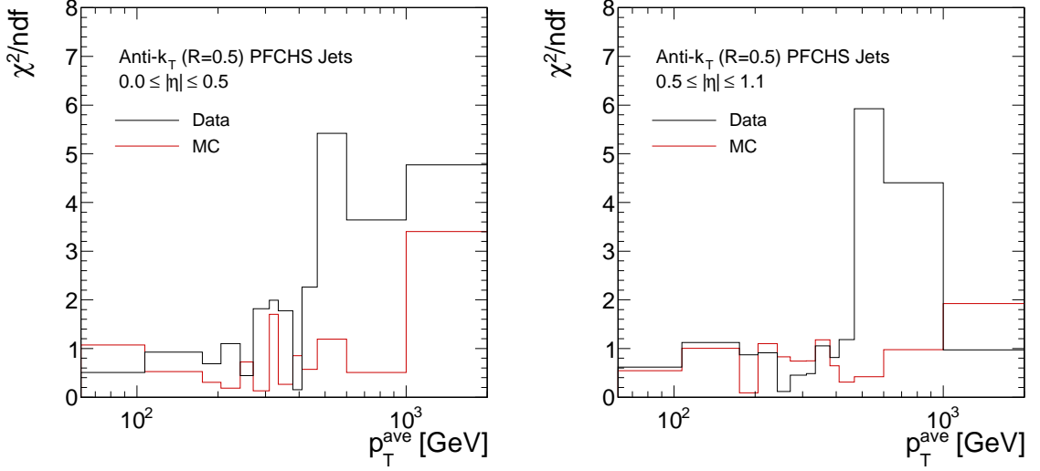
Figure 6.7: Goodness-of-fit test for the extrapolation fits in data and simulation in the two central |\eta| regions as a function of p_T^{\text{ave}} .
