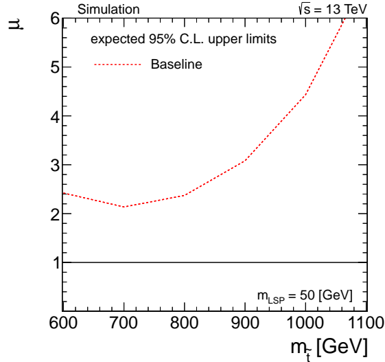
Figure 8.3: Expected 95% C.L. upper limit for signal strength versus m_{\tilde{t}} . The LSP mass is chosen to be 50 GeV.
