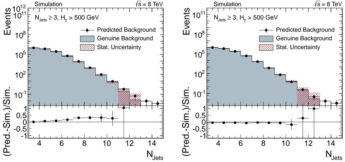
Figure 7.11: Prediction of QCD background on a QCD multijet sample generated with MADGRAPH compared to the expectation from full simulation with a p_T cut of 10 GeV imposed on jets considered in the rebalancing. The predicted N_{\text{jets}} distribution is obtained using the R+S method as in previous versions of the analysis ( left ) and using the R+S method with a correction of the rebalancing step as described in the text ( right ).
