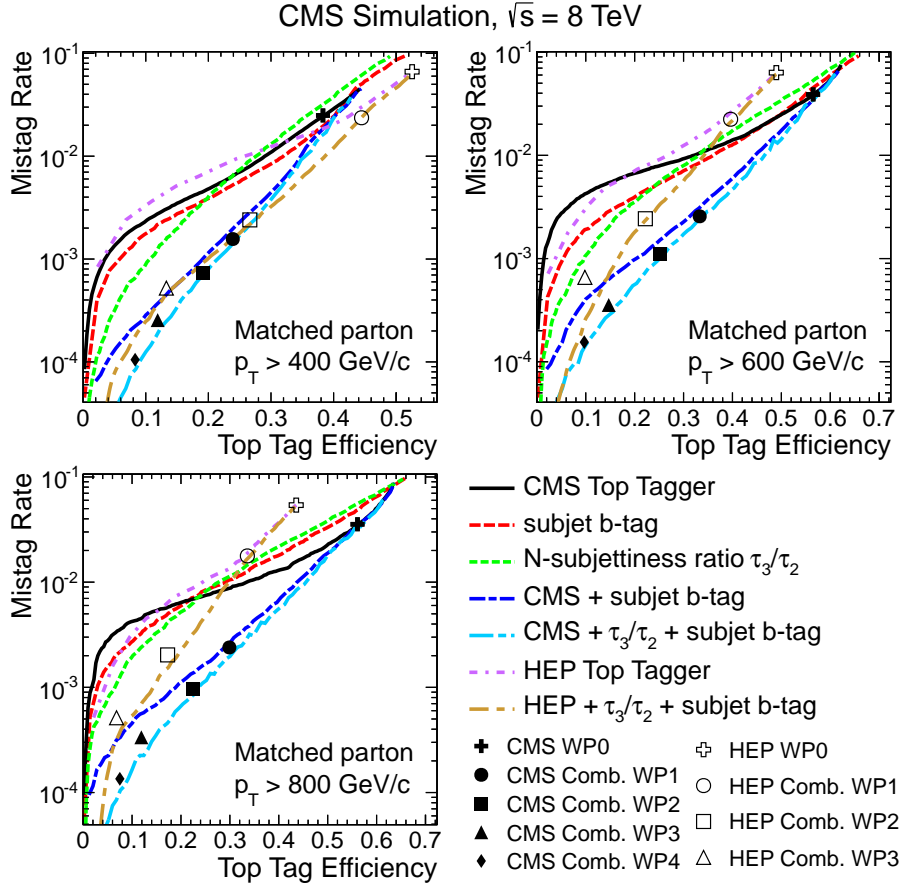
Figure 5.9: Mistag rate versus top-tagging efficiency as measured from QCD PYTHIA6 and POWHEG t\bar{t} simulated events, respectively. In the cases where a jet mass cut is applied, the cut is not varied, but fixed at 140 < m_{\text{jet}} < 250 GeV. N-subjettiness is calculated using R = 0.8 jets except when used in combination with the HEP Top Tagger in which case R = 1.5 jets are used. Signal jets are matched to simulated hadronic generated top quarks, while background jets are matched to simulated partons from the hard scatter. Distributions are shown for three p_T selections, where the p_T cut is applied to the matched generated parton [140].
