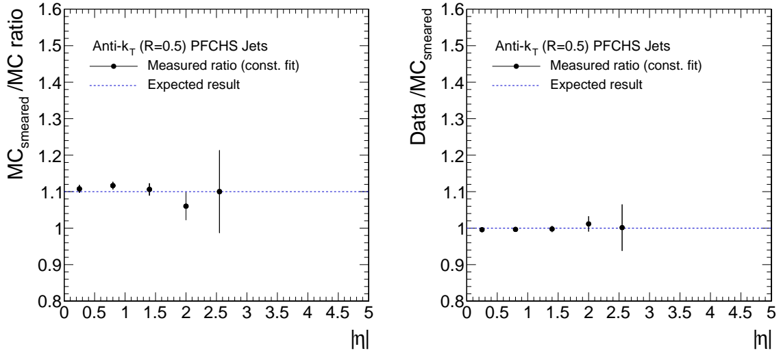
Figure 6.11: Ratio c(MC_{\text{smeared}}/MC) of the resolution in the smeared QCD sample to the resolution of the unsmeared QCD sample as a function of |\eta| with statistical uncertainty ( left ) and ratio c(Data/MC_{\text{smeared}}) of the resolution in data to the resolution of the QCD sample smeared with the measured data-to-simulation ratio as a function of |\eta| with statistical uncertainty ( right ). The blue dashed line indicates the target value of each validation test.
