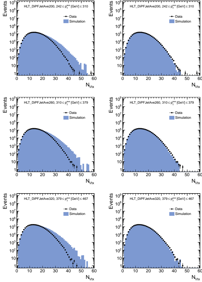
Figure A.2: Distribution of number of primary vertices in data (black dots) and simulation (blue histogram) before ( left ) and after ( right ) reweighting of the pileup scenario in simulation for trigger paths HLT_DiPFJetAve200 ( top ), HLT_DiPFJetAve260 ( middle ) and HLT_DiPFJetAve320 ( bottom ).
