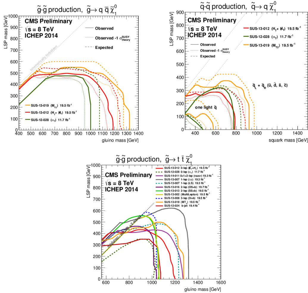
Figure 7.22: Comparison of various exclusion limits derived by different CMS analyses for the process \tilde{g} \rightarrow q\bar{q} + \tilde{\chi}_1^0 (top left), \tilde{q} \rightarrow q + \tilde{\chi}_1^0 (top right) and \tilde{g} \rightarrow t\bar{t} + \tilde{\chi}_1^0 (bottom). Taken from [76].
