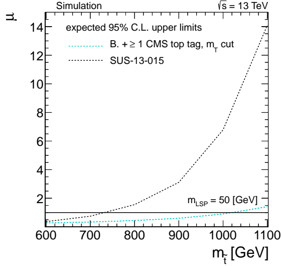
Figure 8.16: Expected 95% C.L. upper limit for signal strength versus m_{\tilde{t}} . The LSP mass is chosen to be 50 GeV. The label B. denotes the baseline selection.
