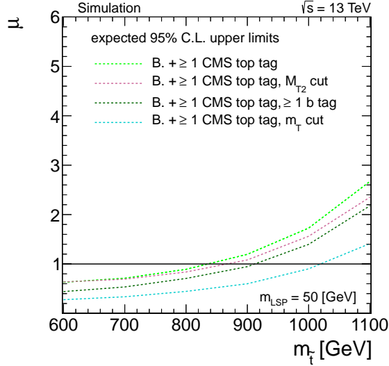
Figure 8.14: Expected 95% C.L. upper limit for signal strength versus m_{\tilde{t}} . The LSP mass is chosen to be 50 GeV. The label B. denotes the baseline selection.
