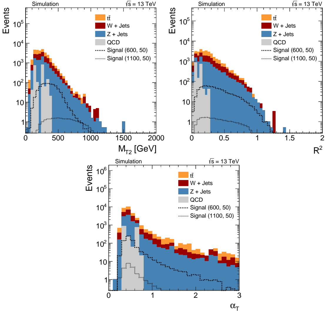
Figure 8.11: Distribution of the M_{T2} ( top left ), the razor variable R^2 ( top right ) and the \alpha_T variable ( bottom ) after application of the baseline selection requirements for background and two selected signal samples. The signal points are labelled as (X, Y) where X is the top squark mass and Y is the LSP mass in GeV.
