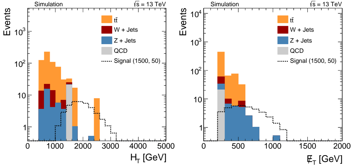
Figure 8.18: Comparison of selected H_T ( left ) and \cancel{E}_T ( right ) distributions in simulated events found from applying the baseline selection criteria, at least one CMS top tag and m_T > 180 GeV. The signal points for gluino-mediated top squark production are labelled as (X, Y) where X is the gluino mass and Y is the LSP mass in GeV.
