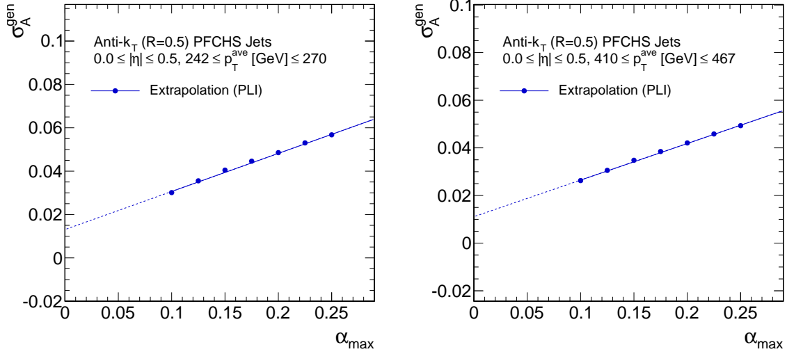
Figure 6.8: Two example extrapolations of measured values for \sigma_A^{\text{gen}} in simulation to determine the contribution from PLI.
