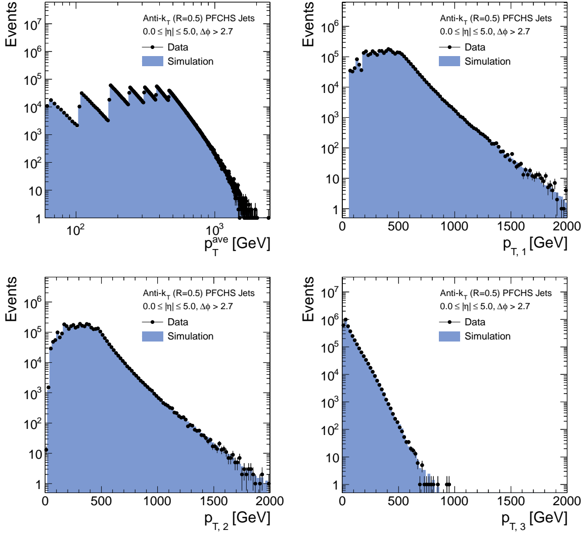
Figure 6.3: Inclusive p_T^{\text{ave}} spectrum of events after the total selection in data and in simulation ( top left ), leading jet p_T ( top right ), subleading jet p_T ( bottom left ) and third jet p_T ( bottom right ).
