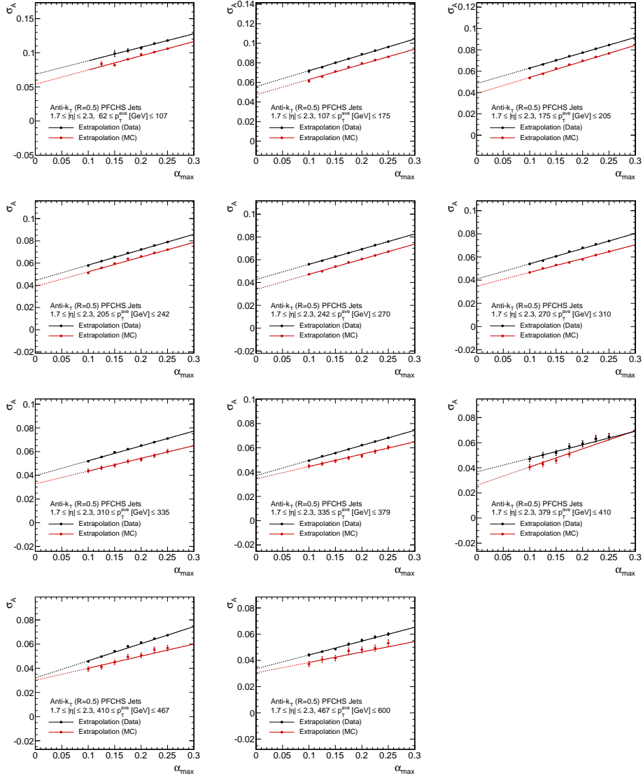
Figure A.6: Extrapolations of measured values for \sigma_A in data and simulation to obtain the result for zero additional jet activity for 1.7 \leq |\eta| \leq 2.3 .
