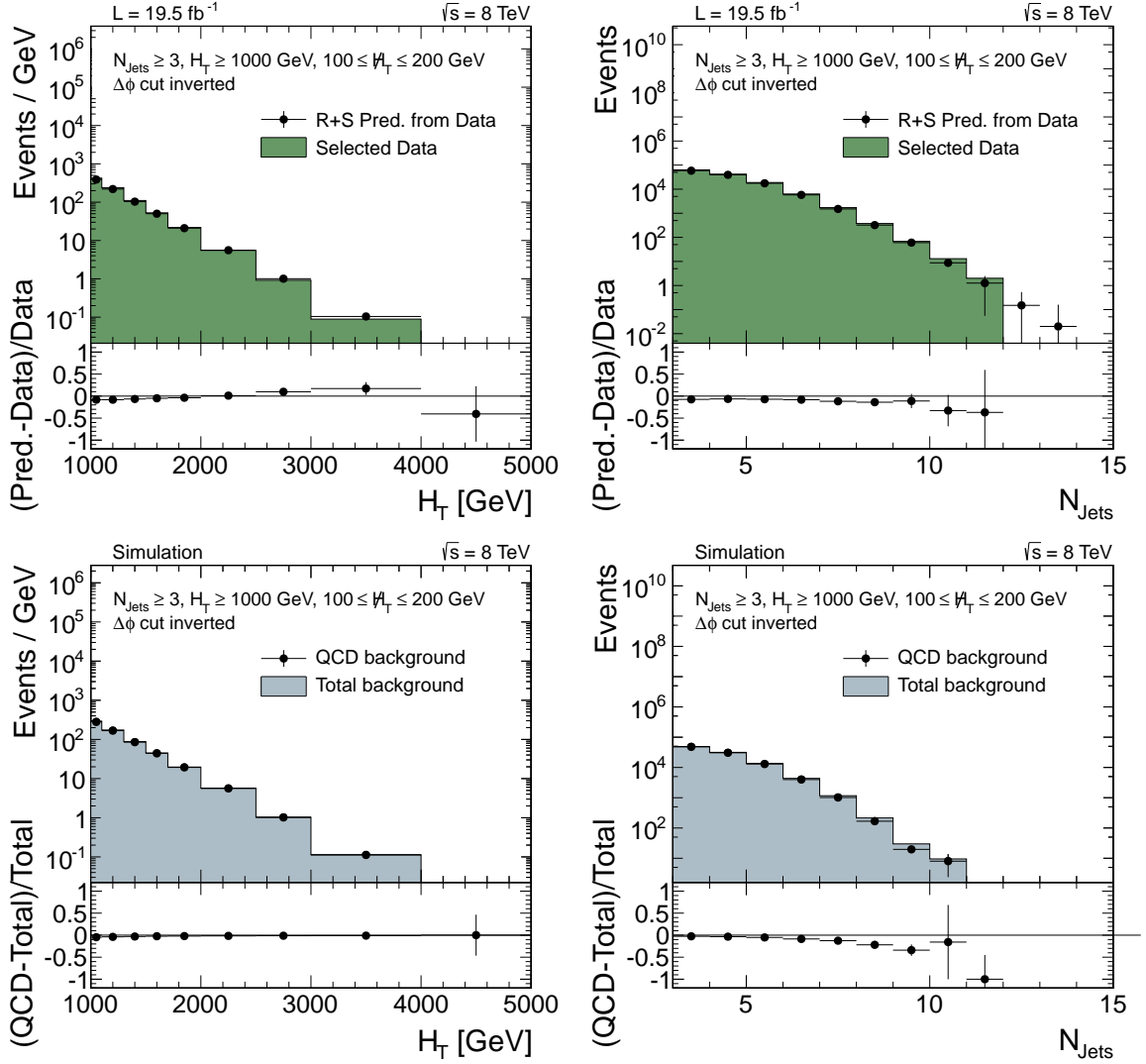
Figure 7.18: Prediction of QCD background on data compared to the expectation from data for a QCD enriched control region with H_T > 1000 GeV, inverted \Delta\phi cut, N_{\text{Jets}} \geq 3 and 100 \leq \cancel{H}_T \leq 200 GeV ( upper row ) and selected QCD events in simulation compared to the total number of selected background events in simulation in the same control region ( lower row ).
