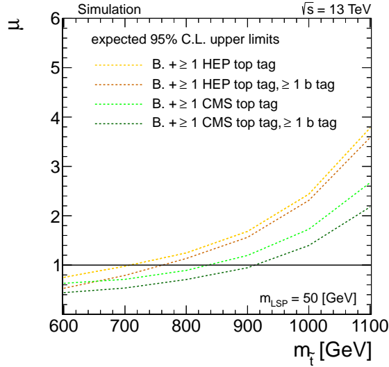
Figure 8.9: Expected 95% C.L. upper limit for signal strength versus m_{\tilde{t}} . The LSP mass is chosen to be 50 GeV. The label B. denotes the baseline selection.
