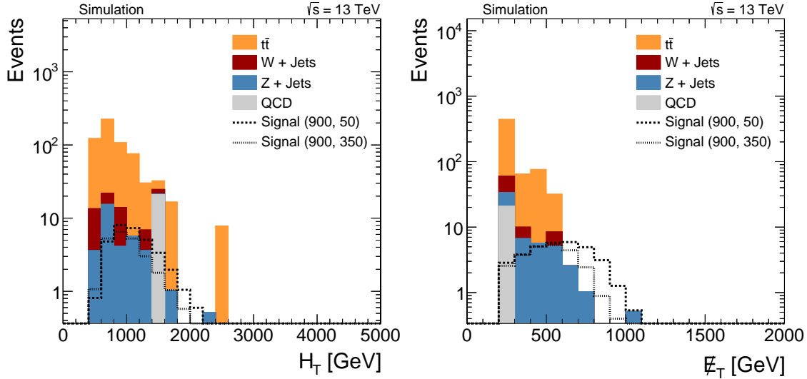
Figure 8.20: Comparison of selected H_T ( left ) and \cancel{E}_T ( right ) distributions in simulated events found from applying the baseline selection criteria, at least one CMS top tag and m_T > 180 GeV. The signal points for direct top squark production are labelled as (X, Y) where X is the top squark mass and Y is the LSP mass in GeV.
