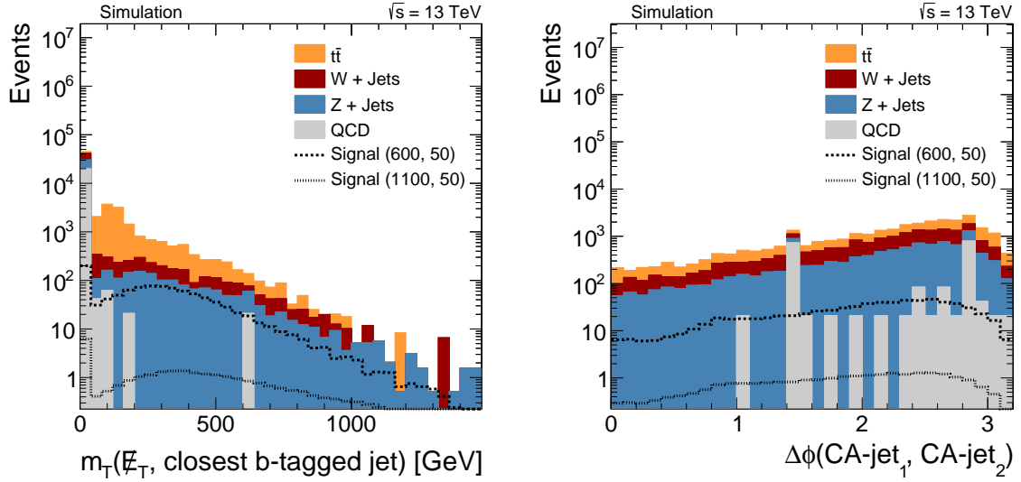
Figure 8.12: Distribution of the m_T variable ( left ) and \Delta\phi(\text{CA-jet}_1, \text{CA-jet}_2) ( right ) after application of the baseline selection requirements for background and two selected signal samples. The signal points are labelled as (X, Y) where X is the top squark mass and Y is the LSP mass.
