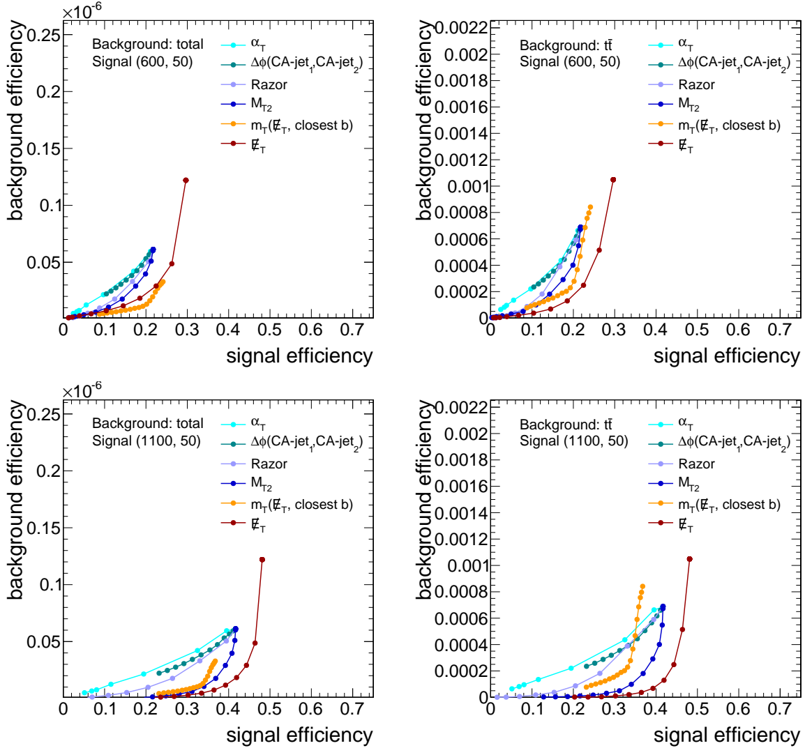
Figure 8.13: Evolution of the signal versus background efficiency for a top squark mass of 600 GeV ( top ) and 1100 GeV ( bottom ) in case the background is the sum of all backgrounds ( left ) or the t\bar{t} background ( right ) after applying baseline selection criteria. The definitions of the variables \alpha_T , \Delta\phi(\text{CA-jet}_1, \text{CA-jet}_2) , razor and M_{T2} imply a requirement of at least two CA-jets and the definition of m_T implies a requirement of at least one b-tagged jet.
