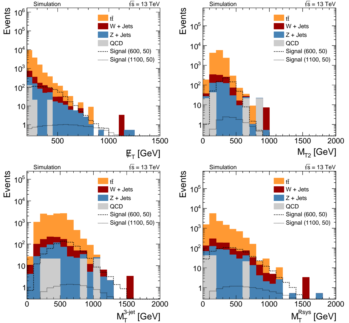
Figure 8.15: Comparison of E_T , M_{T2} , M_T^{3\text{-jet}} and M_T^{\text{Rsys}} distributions for signal and background events after applying preselection criteria and E_T > 200 GeV. The signal points are labelled as (X, Y) where X is the top squark mass and Y is the LSP mass in GeV.
