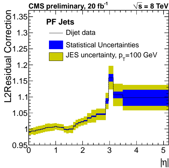
Figure 5.6: L2 residual corrections for AK5 PF jets as a function of jet pseudorapidity, obtained from dijet events, shown with JES uncertainty (yellow band) and the statistical uncertainty (blue band) [136].
