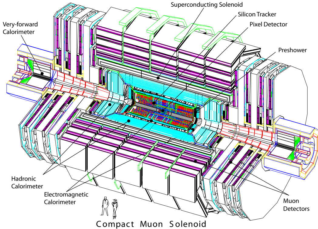
Figure 3.3: A perspective view of the CMS detector [92].
