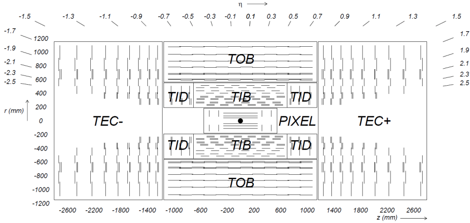
Figure 3.4: Sketch of the CMS tracking system in a rz -view. Each tracker module is represented by one line [92].
