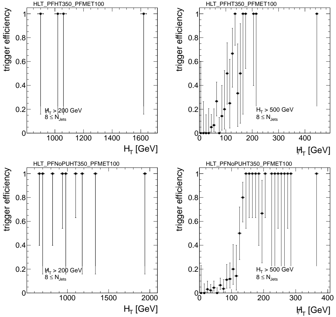
Figure B.2: Measured relative trigger efficiency for paths HLT_PFHT350_PFMET100 (top) and HLT_PFN0PUHT350_PFMET100 (bottom) as a function of H_T (left) and \#H_T (right) shown for 8 \leq N_{\text{Jets}} .
