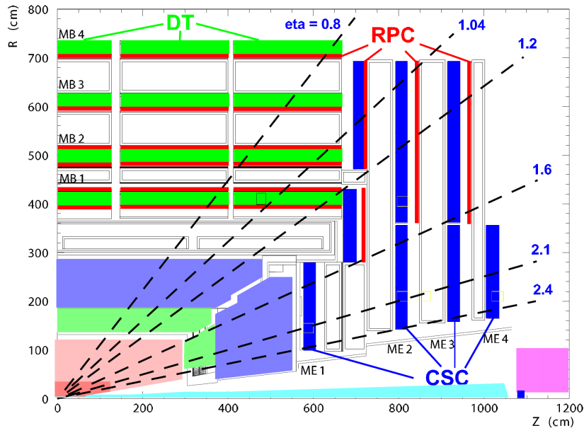
Figure 3.7: View of one quarter section of the muon system in the rz -plane [93].
