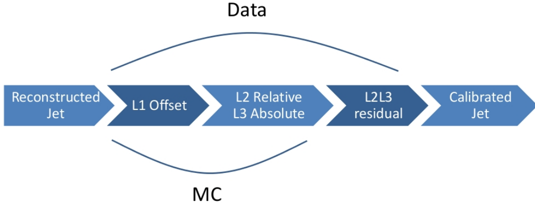
Figure 5.3: Sketch of the factorized approach used for jet energy corrections at the CMS experiment.
