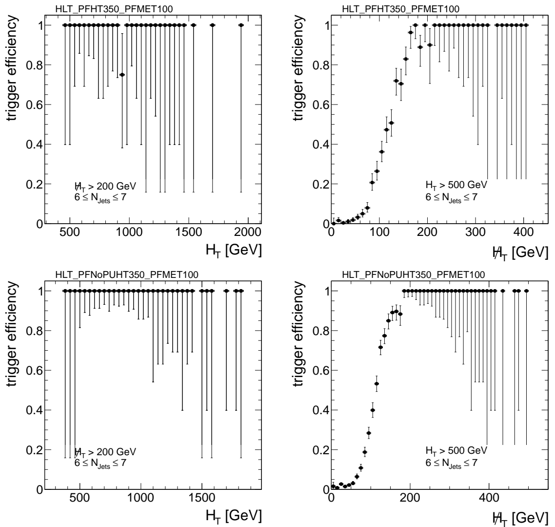
Figure B.1: Measured relative trigger efficiency for paths HLT_PFHT350_PFMET100 (top) and HLT_PFN0PUHT350_PFMET100 (bottom) as a function of H_T (left) and \#H_T (right) shown for 6 \leq N_{\text{Jets}} \leq 7 .
