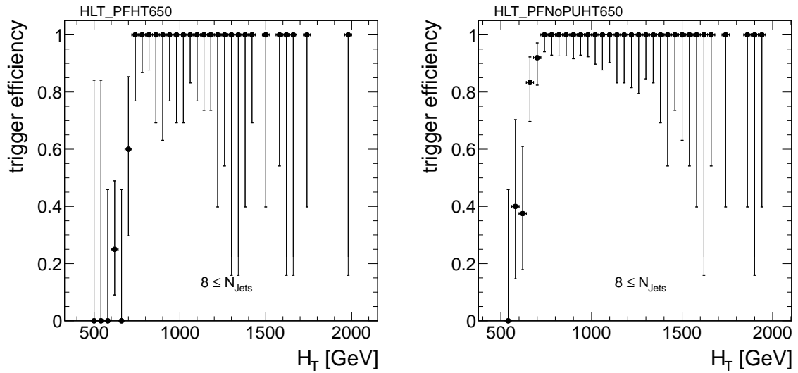
Figure B.6: Measured trigger efficiency for paths HLT_PFHT650 ( left ) and HLT_PFNoPUHT650 ( right ) as a function of H_T illustrated for N_{\text{Jets}} \geq 8 .
