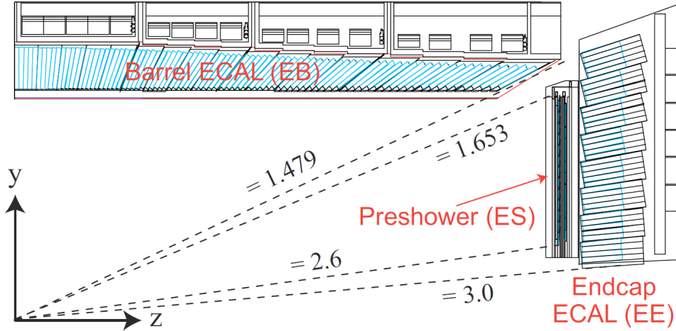
Figure 3.5: View of one quarter section of the CMS electromagnetic calorimeter in a yz -view [93].
