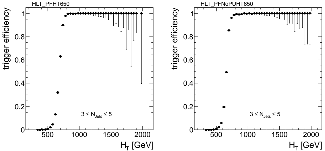
Figure 7.16: Measured trigger efficiency for paths HLT_PFHT650 ( left ) and HLT_PFN0PUHT650 ( right ) as a function of H_T , shown for 3 \leq N_{\text{Jets}} \leq 5 .
