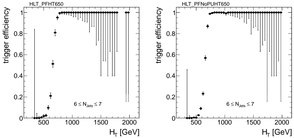
Figure B.5: Measured trigger efficiency for paths HLT_PFHT650 ( left ) and HLT_PFNoPUHT650 ( right ) as a function of H_T illustrated for 6 \leq N_{\text{Jets}} \leq 7 .
