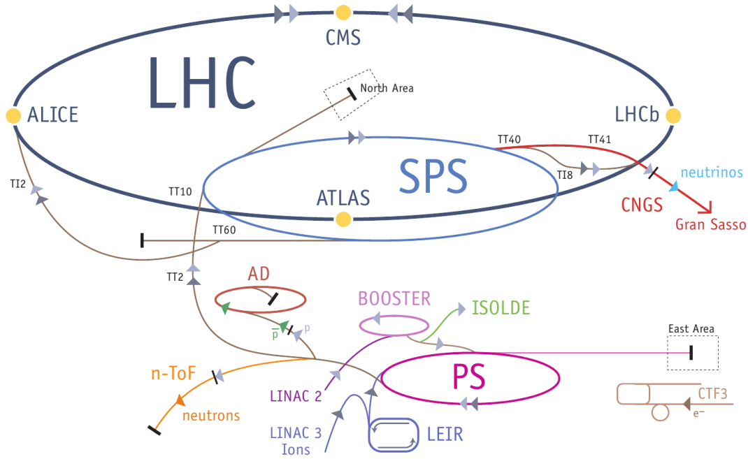
Figure 3.1: Illustration of the CERN accelerator complex including the injector chain of the LHC ring [89].
