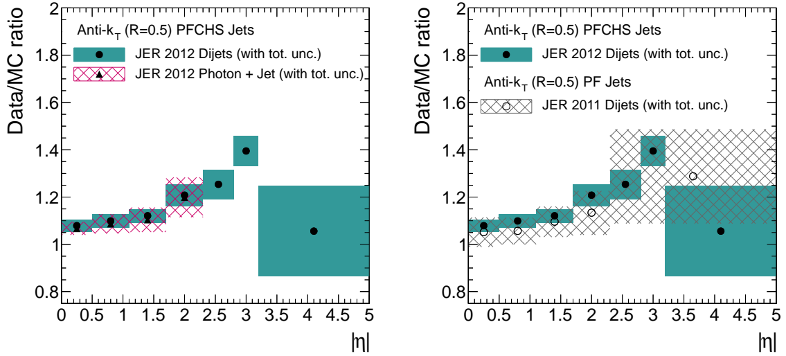
Figure 6.19: Measured data-to-simulation ratio in various |\eta| regions displayed with total uncertainty. Comparison to results obtained for \sqrt{s} = 8 TeV data from \gamma + \text{jet} events ( left ) and to \sqrt{s} = 7 TeV data from dijet events ( right ).
