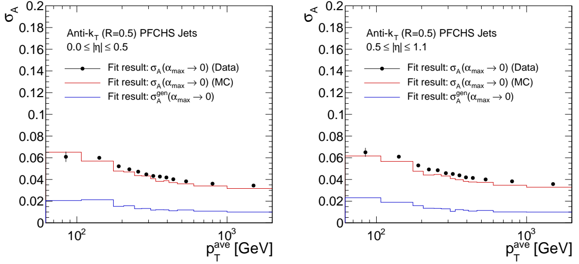
Figure 6.9: Results of extrapolation fits in the two central |\eta| regions as a function of p_T^{\text{ave}} for data (black), simulation (red) and particle-level imbalance (blue).
