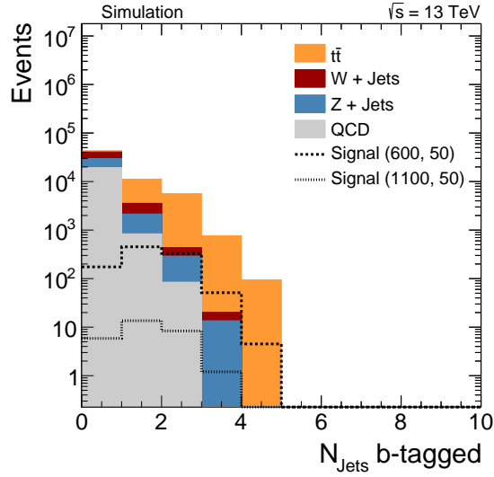
Figure 8.4: B-tag multiplicity after applying the baseline selection in simulated events. The signal points are labelled as (X, Y) where X is the top squark mass and Y is the LSP mass in GeV.
