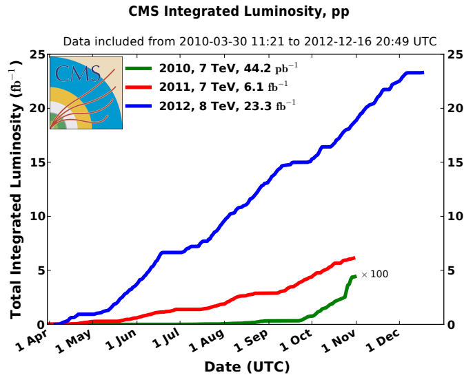
Figure 3.8: Cumulative integrated luminosity versus day delivered to CMS during stable beams for pp collisions. Different data-taking periods are indicated as follows: 2010 (green), 2011 (red) and 2012 (blue) [100].
