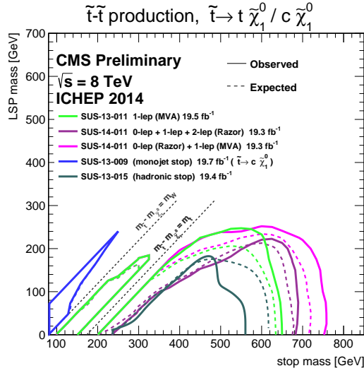
Figure 7.24: Exclusion limits derived by different CMS analyses for the process \tilde{t} \rightarrow t\tilde{\chi}_1^0 in the m_{\tilde{t}} versus m_{\text{LSP}} plane. Taken from [76].
