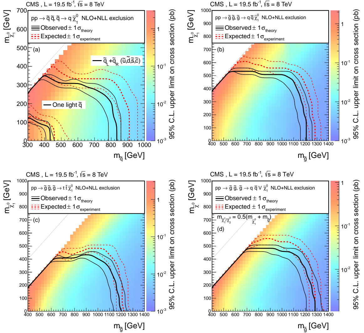
Figure 7.21: The observed and expected 95% C.L. upper limits on the (a) squark-squark and (b–d) gluino-gluino production cross sections in either the m(\text{squark}) - m(\text{LSP}) or the m(\text{gluino}) - m(\text{LSP}) plane obtained with the simplified models. For the squark-squark production the upper set of curves corresponds to the scenario when the first two generations of squarks are degenerate and light, while the lower set corresponds to only one light accessible squark [168].
