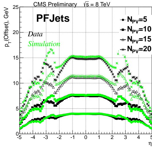
Figure 5.4: L1 offset transverse momentum correction for AK5 PF jets as a function of jet pseudorapidity in data (black) and simulation (green). Different intervals of reconstructed primary vertices ( N_{PV} ) are shown with different markers [136].
