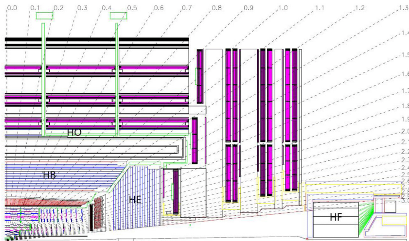
Figure 3.6: Longitudinal view of one quarter of the CMS detector showing the location of the individual HCAL sub-detector parts [92].
