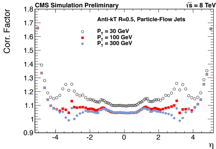
Figure 5.5: MC-Truth corrections for AK5 PF jets as a function of jet pseudorapidity for three reference transverse momentum values: 30 GeV (white hollow circles), 100 GeV (red squares) and 300 GeV (blue circles) [136].
