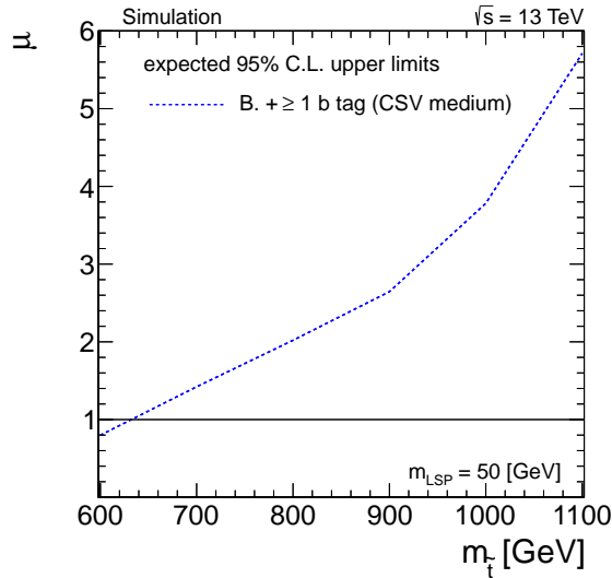
Figure 8.5: Expected 95% C.L. upper limit for signal strength versus m_{\tilde{t}} . The LSP mass is chosen to be 50 GeV. The label B. denotes the baseline selection.
