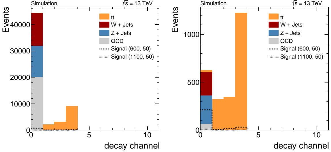
Figure 8.10: Comparison of decay modes of signal and background processes defined according to the top quark properties based on generator information after the baseline selection ( left ) and after the baseline selection and the requirement of \geq 1 CMS top tag ( right ). For a definition of the decay channels see text.
