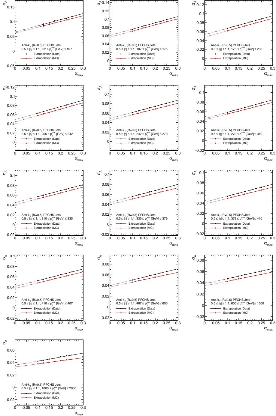
Figure A.4: Extrapolations of measured values for \sigma_A in data and simulation to obtain the result for zero additional jet activity for 0.5 \leq |\eta| \leq 1.1 .
