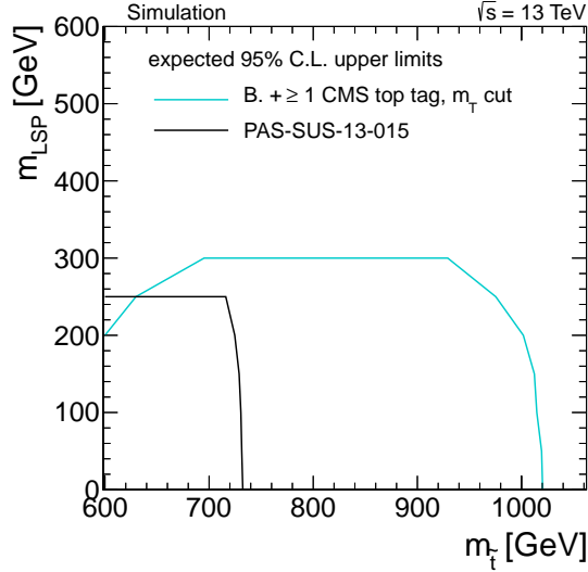
Figure 8.21: Expected 95% C.L. upper limit for m_{\tilde{t}} versus m_{\text{LSP}} . The label B. denotes the baseline selection.
