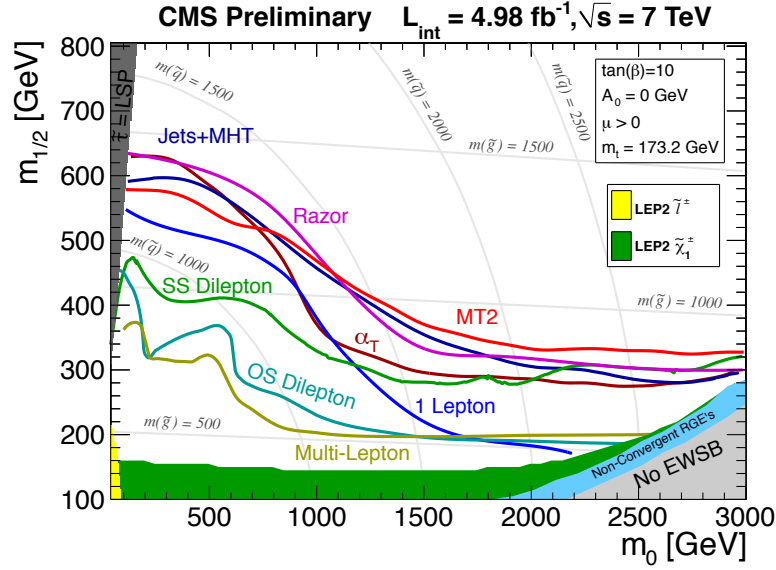
Figure 2.7: Interpretation of searches for supersymmetry at the CMS experiment within the CMSSM. Shown are the 95% C.L. exclusion limits in the m_0 and m_{1/2} plane for various searches performed using different final state topologies [76].
