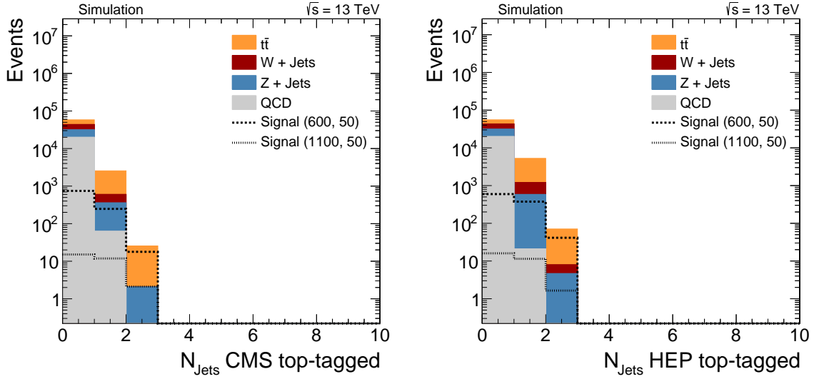
Figure 8.8: Top-tag multiplicity for the CMS Top Tagger ( left ) and the HEP Top Tagger ( right ) after application of the baseline selection. Only CA-jets of the corresponding jet size with a transverse momentum above 150 GeV are considered.
