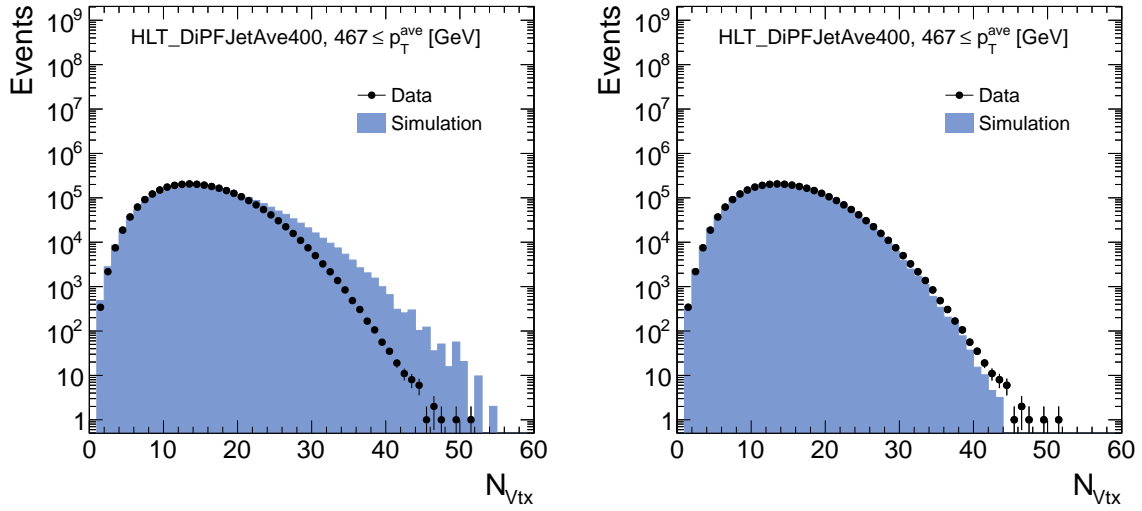
Figure 6.2: Distribution of number of primary vertices in data (black dots) and simulation (blue histogram) before ( left ) and after ( right ) reweighting of the pileup scenario in simulation for trigger path HLT_DiPFJetAve400.
