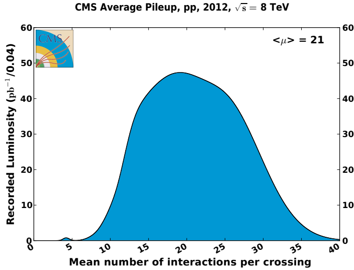
Figure 3.9: Mean number of interactions per bunch crossing in pp collisions at a centre-of-mass energy of \sqrt{s} = 8 TeV [100].
