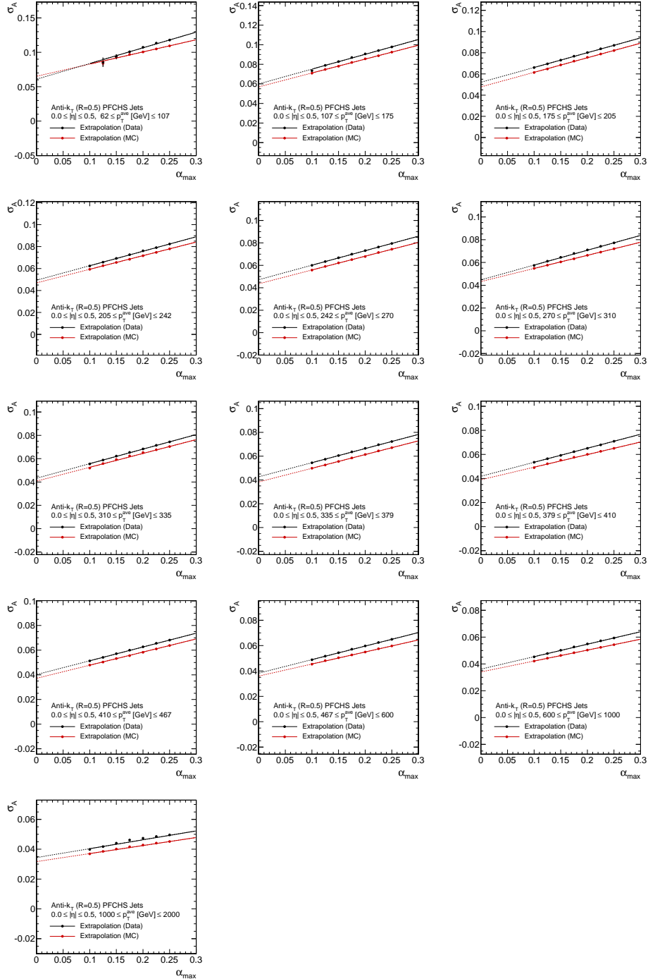
Figure A.3: Extrapolations of measured values for \sigma_A in data and simulation to obtain the result for zero additional jet activity for 0.0 \leq |\eta| \leq 0.5 .
