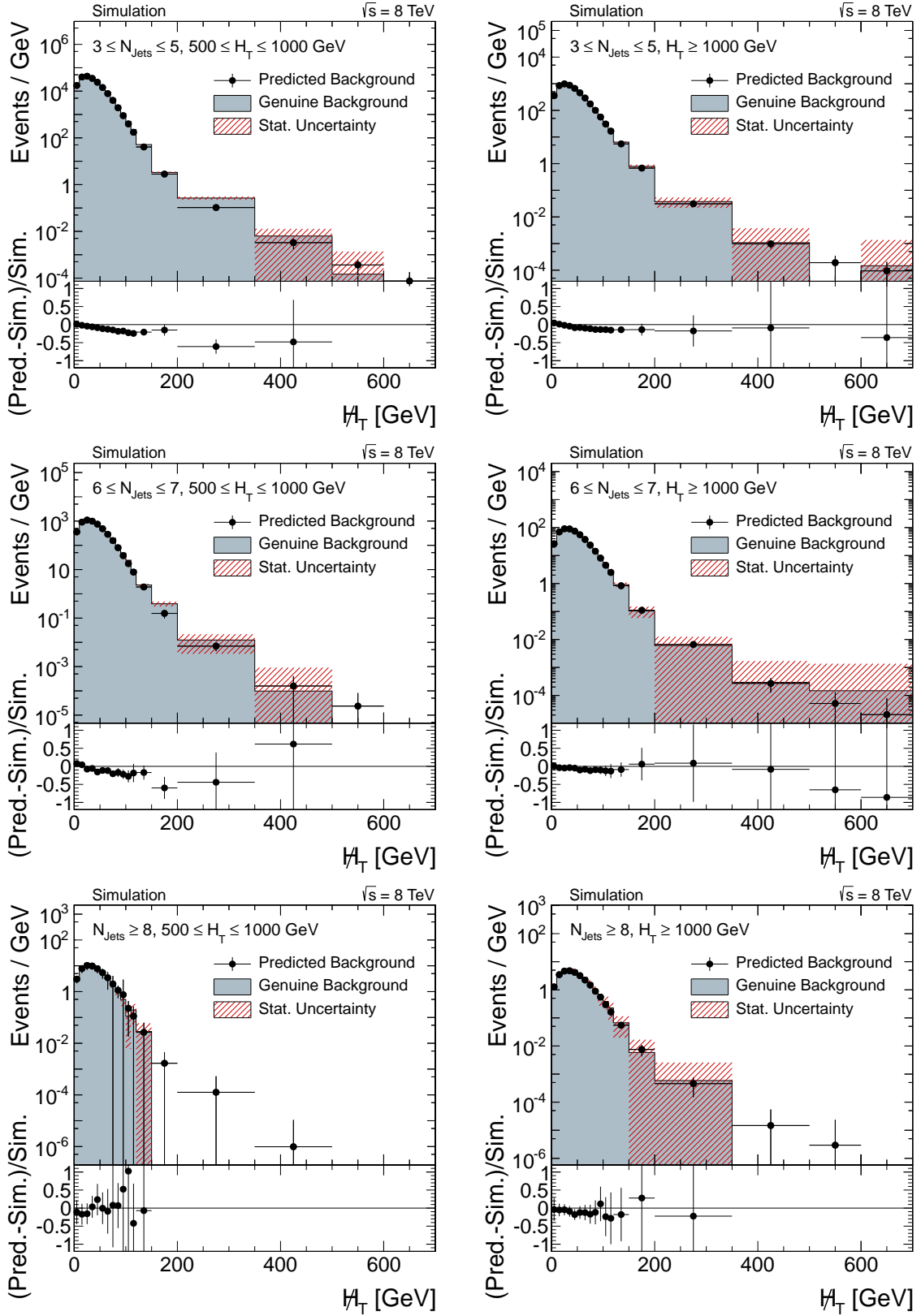
Figure 7.14: Prediction of QCD background on a QCD multijet sample generated with MADGRAPH compared to the expectation from full simulation. The closure test is shown for various jet multiplicity bins and low (left) or high (right) H_T selections.
