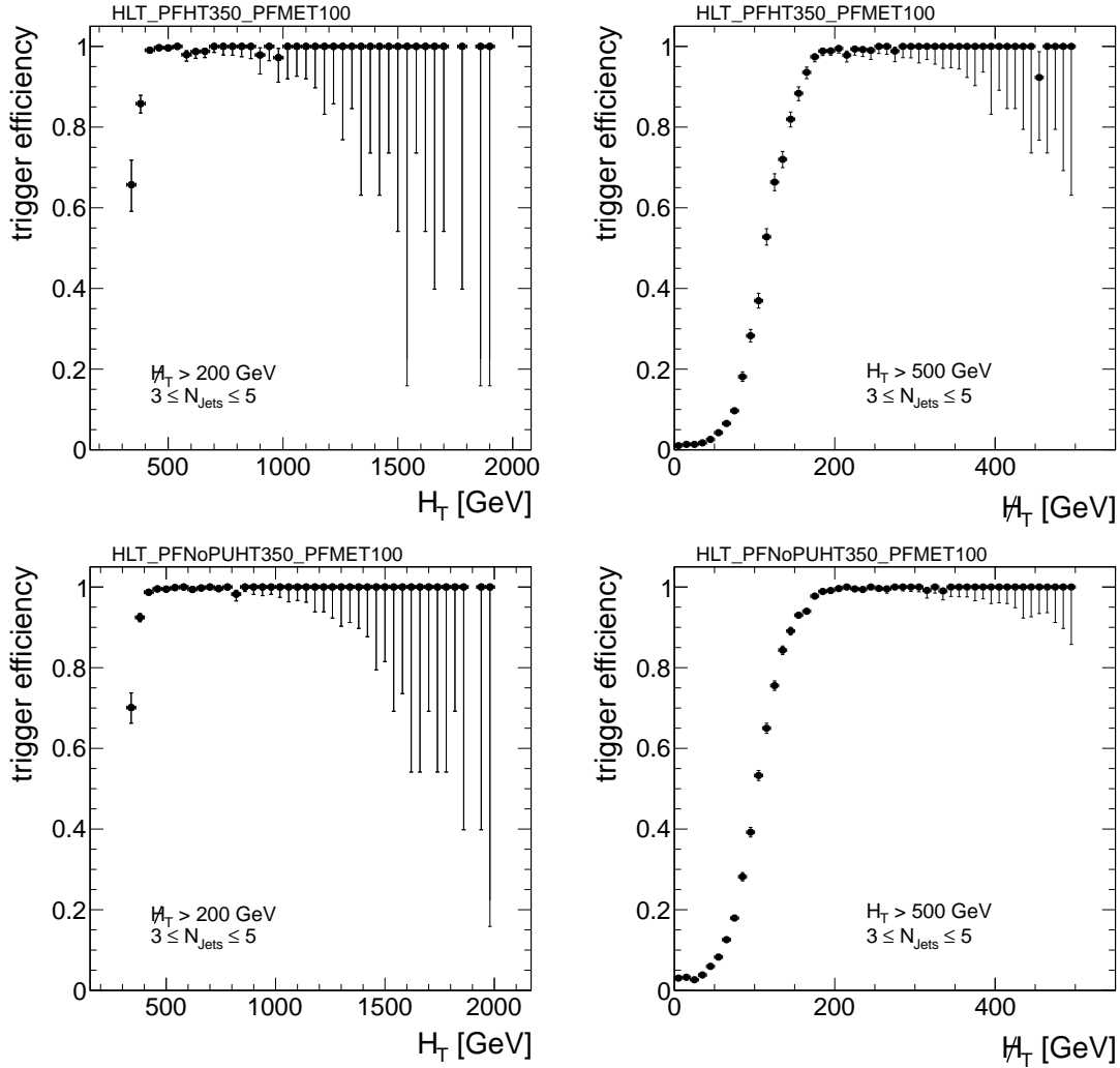
Figure 7.2: Measured relative trigger efficiency for paths HLT_PFHT350_PFMET100 ( top ) and HLT_PFN0PUHT350_PFMET100 ( bottom ) as a function of H_T ( left ) and \#H_T ( right ) shown for 3 \leq N_{\text{Jets}} \leq 5 .
