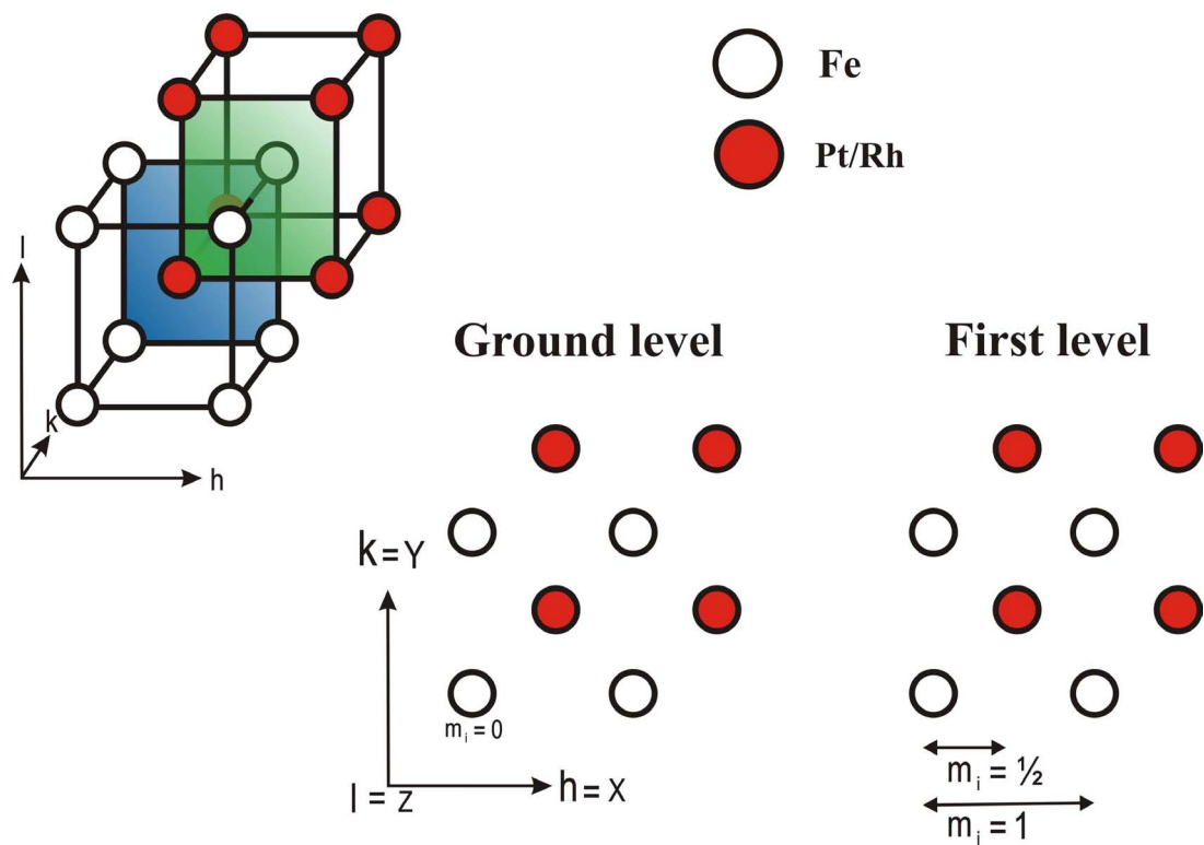
Figure 5.10.: Magnetic unit cell of the bct structure. The right side shows the top view on the bct structure. The Fe and Pt/Rh atoms in the ground and first level have different positions in z -direction as can be seen in the sketch on the left side. For more details see the text.
