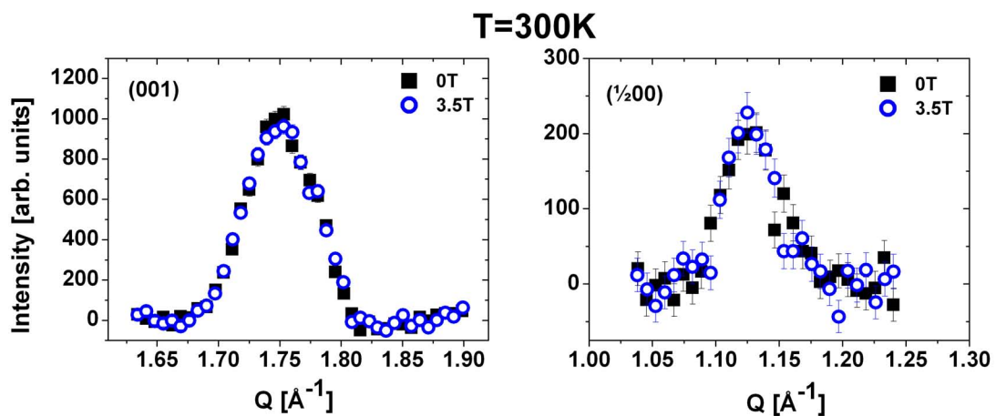
Figure 5.36.: Magnetic field dependence of the (001) and (\frac{1}{2}00) reflection of the \text{Fe}_{50}\text{Pt}_{32.5}\text{Rh}_{17.5} film at T=300\text{ K} for 0 T (black squares) and 3.5 T (open circles). The external magnetic field was applied in-plane along the b-axis.
