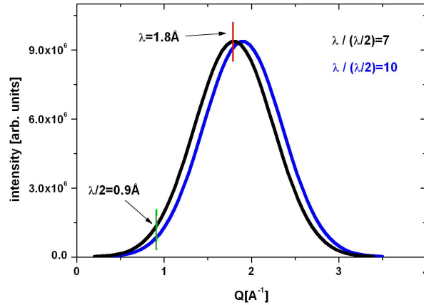
Figure 4.5.: Schematic sketch of the effect of the wavelength offset for the velocity selector. The black and blue lines are the intensity distributions behind the selector without and with the wavelength offset.
