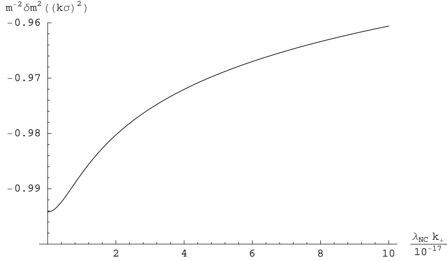
Figure 5.1.: The relative mass correction m^{-2}\delta m^2((k\sigma)^2) as a function of the perpendicular momentum k_{\perp} .
