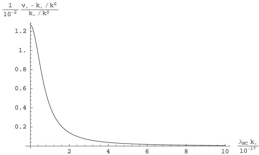
Figure 5.2.: The distortion of the group velocity in perpendicular direction as a function of the perpendicular momentum k_{\perp} .
