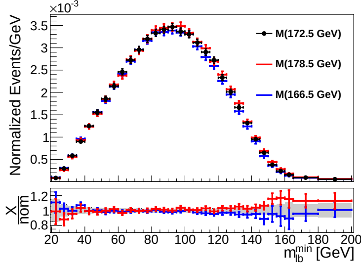
Figure 6.10: Folded and normalized m_{\text{lb},\text{pred}}^{\text{min}} distribution as predicted by MADGRAPH+PYTHIA for m_t^{\text{MC}} = 172.5 GeV. The folding is performed with the response matrix M corresponding to m_t^{\text{MC}} = 172.5 GeV (nominal), m_t^{\text{MC}} = 178.5 GeV, or m_t^{\text{MC}} = 166.5 GeV. The statistical uncertainties are indicated with error bars. The lower panel shows the ratio of all distributions with respect to the nominal one. For the latter, statistical uncertainties are indicated with a shaded band.
