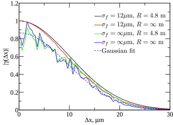
Figure 5.20: The impact of the wavefront curvature on the analysis of the URA diffraction patterns. The "experimental" diffraction pattern I(\mathbf{q}) in (5.7) is calculated using a Gaussian Schell-model beam with \xi_f = 10 \mu\text{m} , \sigma_f = 12 \mu\text{m} , and R = 4.8 \text{ m} . The coherent ( \xi_f = \infty ) diffraction pattern I_{\text{coh}}(\mathbf{q}) was simulated with \sigma_f = 12 \mu\text{m} and R = 4.8 \text{ m} (black solid line), \sigma_f = 12 \mu\text{m} and R = \infty \text{ m} (red solid line), \sigma_f = \infty \mu\text{m} and R = 4.8 \text{ m} (green solid line), and \sigma_f = \infty \mu\text{m} and R = \infty \text{ m} (blue solid line). A Gaussian fit to the blue circles is shown by the blue dashed line.
