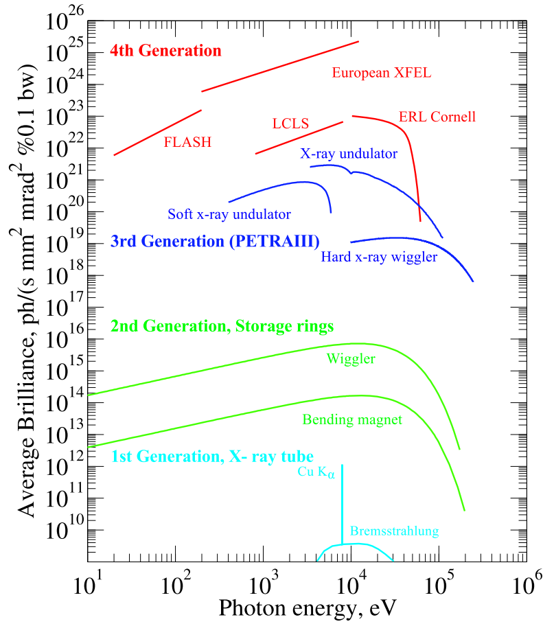
Figure 1.1: Average brilliance of available and planned x-ray radiation sources as a function of photon energy. Third and fourth generation sources situated at DESY (PETRA III, FLASH and European XFEL), the first operating hard x-ray FEL LCLS in Stanford and the planned ERL in Cornell are shown. For comparison the brilliance from the first and second generation sources is also shown. All plots were taken from [3], except for the planned linear undulator source at an ERL [9].
