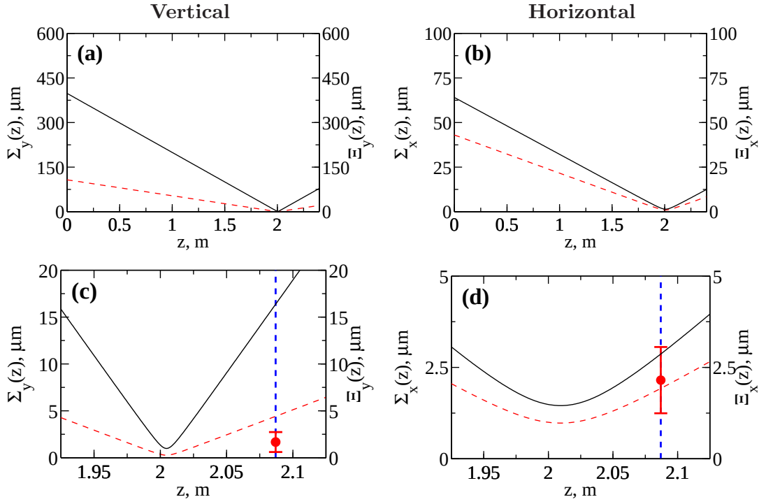
Figure 4.4: Focusing properties of the transfocator with three beryllium lenses at P10 beamline (PETRA III) at an energy of 7.9 keV. The beam size \Sigma(z) (red dashed line) and the transverse coherence length \Xi(z) (black line) are presented. The focusing in the vertical direction (a) and in the horizontal direction (b) are shown. The magnified region near the focal position is presented in (c) and (d). The results from the beam size measurements at the position indicated by the blue dashed line are shown by red dots.
