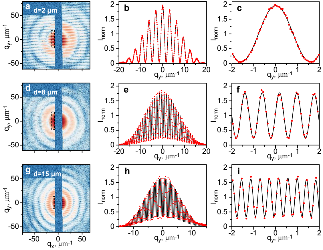
Figure 5.2: Measured diffraction patterns. Left column: Interference fringes from pinholes separated by (a) 2\ \mu\text{m} , (d) 8\ \mu\text{m} and (g) 15\ \mu\text{m} each exposed to a single shot of the LCLS beam as a function of the transverse momentum transfer q_x , q_y . The area used for the analysis of the transverse coherence is shown by the dashed black rectangle close to the center of the patterns. Middle column: Line scans of the interference fringes on the right edge of the marked region, experimental data (red dots) and results of the theoretical fit (black lines). Right column: enlarged regions of the line scans shown in the middle column.
