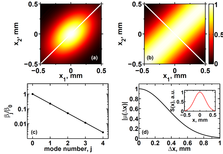
Figure 3.8: Calculations of the coherence properties of the SASE1 undulator at the European XFEL (see Table 3.3) 500 m downstream of the source in the frame of a GSM source. (a) The absolute value of the CSD |W(x_1, x_2)| . (b) The absolute value of the SDC |\mu(x_1, x_2)| . (c) The ratio \beta_j/\beta_0 of the eigenvalue \beta_j to the lowest order eigenvalue \beta_0 as a function of mode number j . (d) The absolute value of the SDC |\mu(\Delta x)| taken along the white line in (b). In the inset the spectral density S(x) is shown that is taken along the white line in (a).
