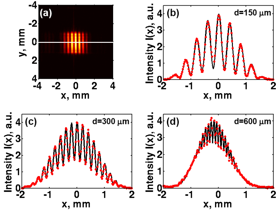
Figure 5.12: Results of a double-slit experiment. (a) A typical data set measured on the detector with vertical slits of 150\text{ }\mu\text{m} separation. Each image is a result of an accumulation of ten pulses. The framed region in the image of three pixels wide was used for further analysis. (b-d) Results of the fit (solid lines) to experimental data (points) for different slit separations d=150\text{ }\mu\text{m} (b), d=300\text{ }\mu\text{m} (c), d=600\text{ }\mu\text{m} (d) in the horizontal direction. The error bars of the data are less than 3 % and are smaller than the symbols used to represent the data. The error metric defined as E = \sum_{i=1}^N (I_i^{\text{exp}} - I_i^{\text{fit}})^2 / \sum_{i=1}^N (I_i^{\text{fit}})^2 was less than 0.002 for all fits.
