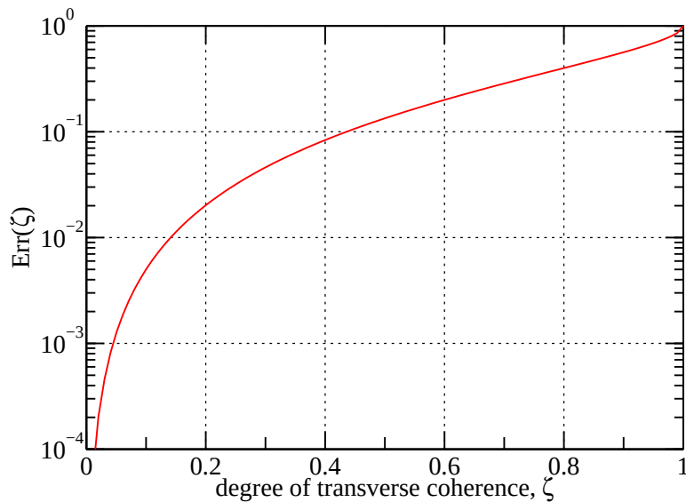
Figure 2.5: The relative error \text{Err}(\zeta) = [\Xi(z) - \Xi_{\text{inc}}(z)] / \Xi(z) between the transverse coherence length determined by the van Cittert- Zernike theorem \Xi_{\text{inc}}(z) and within the GSM \Xi(z) as a function of the degree of transverse coherence \zeta .
