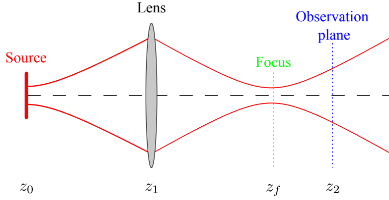
Figure 4.2: The propagation geometry. The source is positioned at z_0 , the lens is at z_1 and the observation plane is at z_2 .
