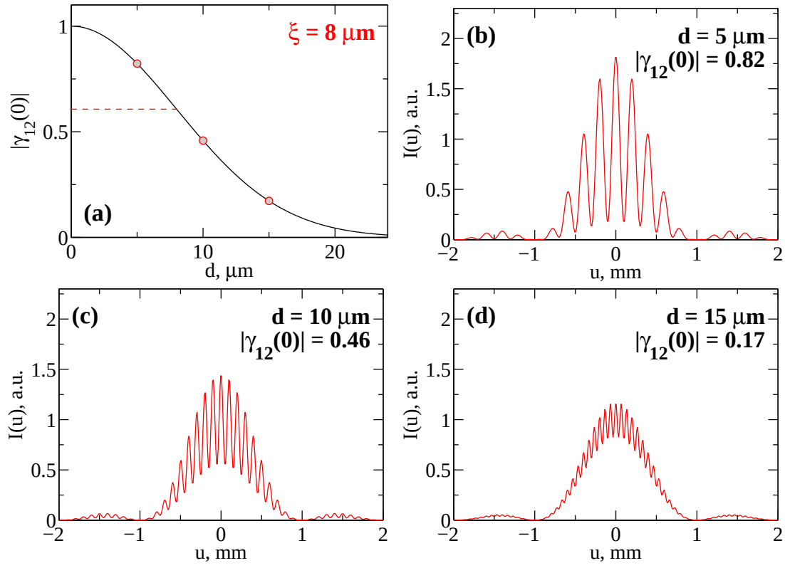
Figure 2.8: Simulated intensity distribution from a double slit experiment for transverse partially coherent radiation. Following parameters were used \lambda = 1 \text{ nm} , slit width a = 1 \text{ }\mu\text{m} , and double slit to detector distance z = 1 \text{ m} . (a) The simulated complex degree of coherence |\gamma_{12}(0)| . (b-d) The intensity distribution on the detector for a slit separation d of 5 \text{ }\mu\text{m} (b), 10 \text{ }\mu\text{m} (c), and 15 \text{ }\mu\text{m} (d). The transverse coherence length is defined by the rms width of |\gamma_{12}(0)| (red dashed line in (a)). Temporally coherent radiation has been assumed in this simulation.
